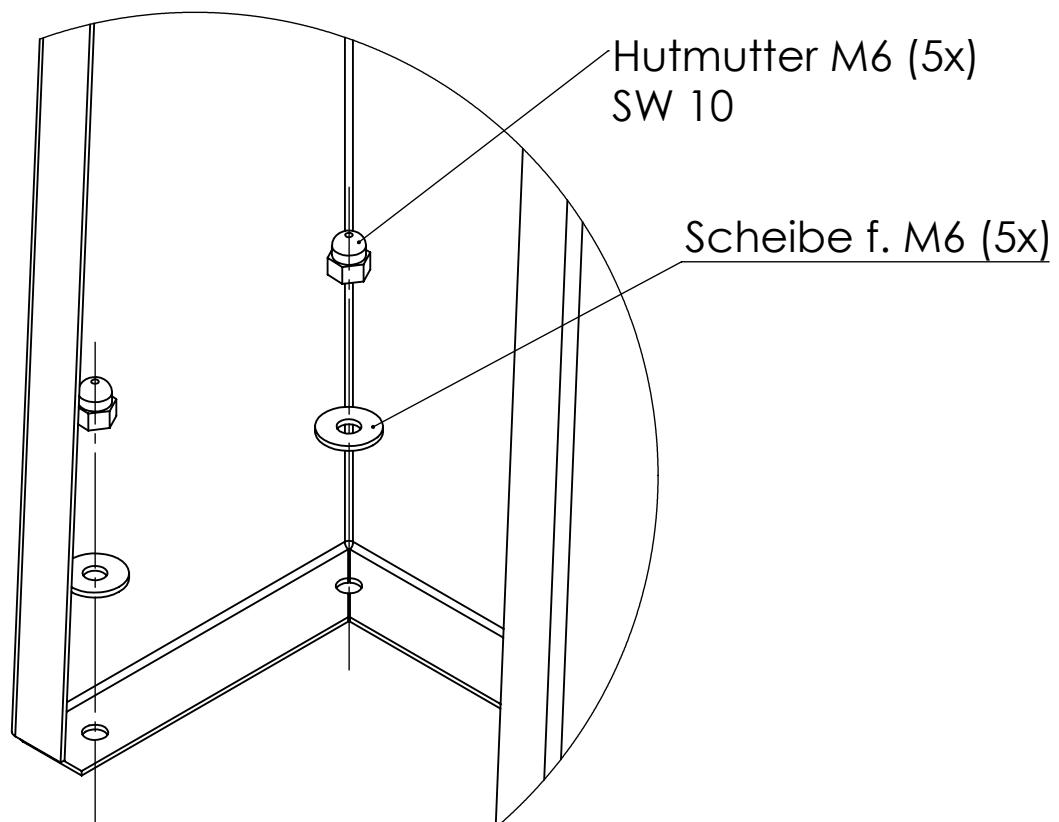
Detail A
